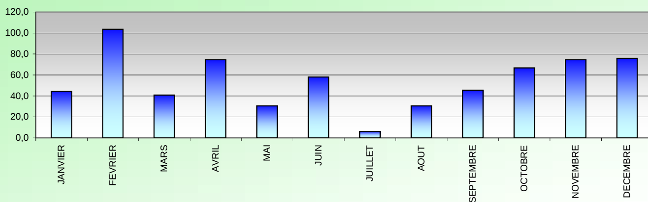
PRECIPITATIONS (mm) 2009
