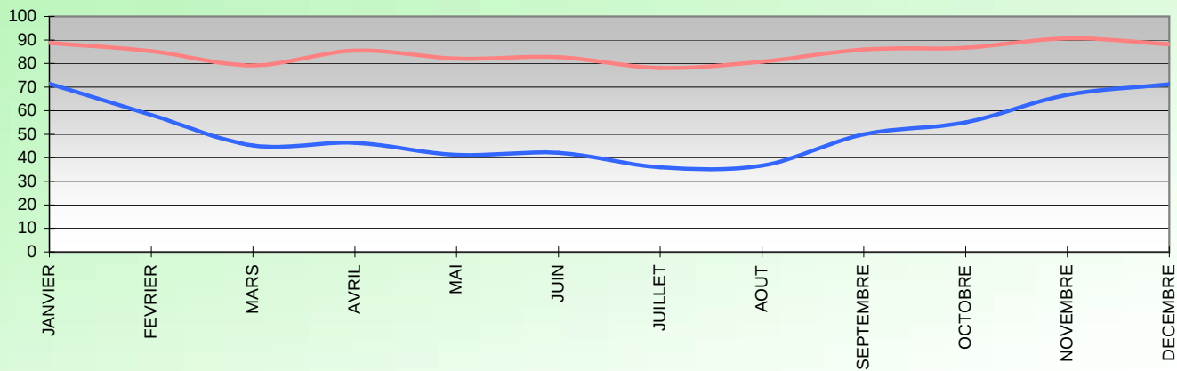
HUMIDITE RELATIVE (%) 2009
