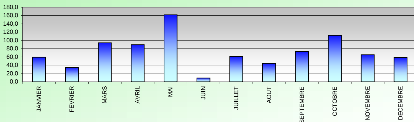
PRECIPITATIONS (mm) 2013
