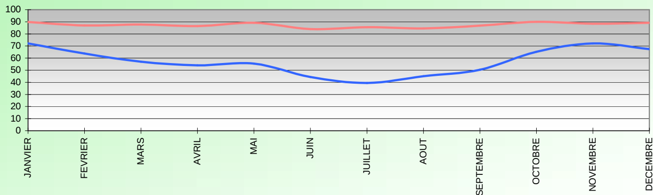
PRECIPITATIONS (mm) 2013
