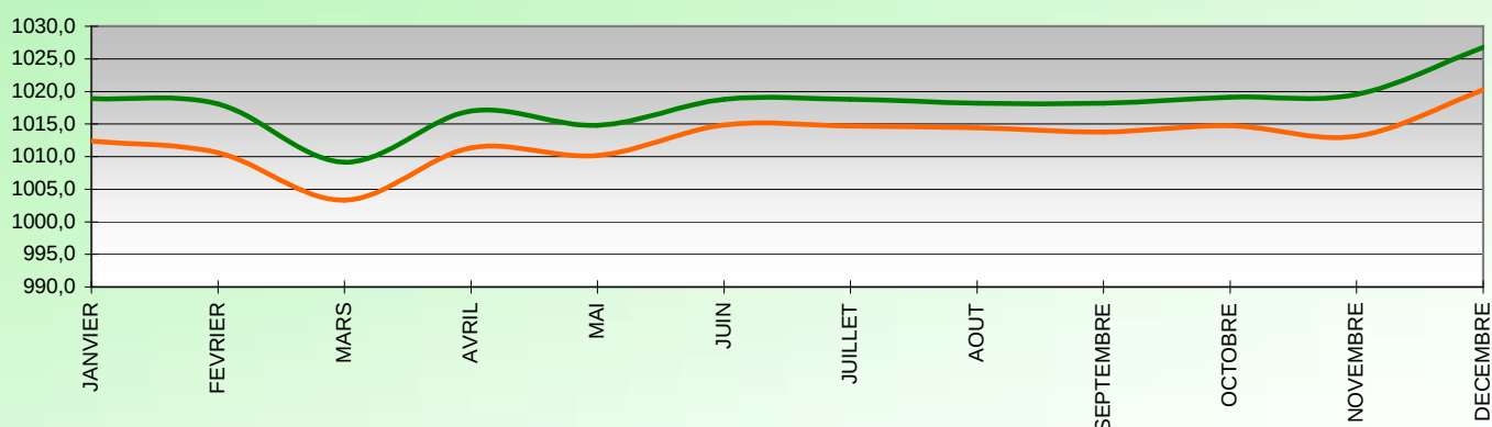
HUMIDITE RELATIVE (%) 2013
