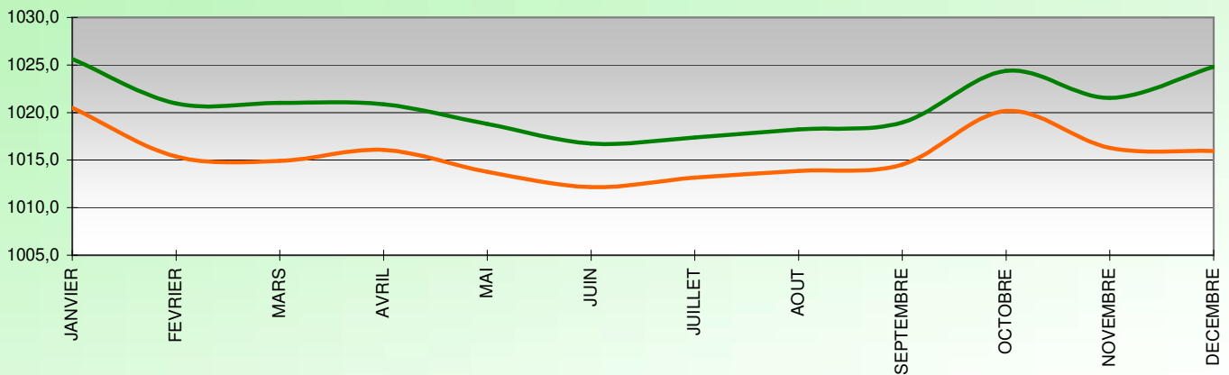
PRESSION RELATIVE (hPa) 2017
