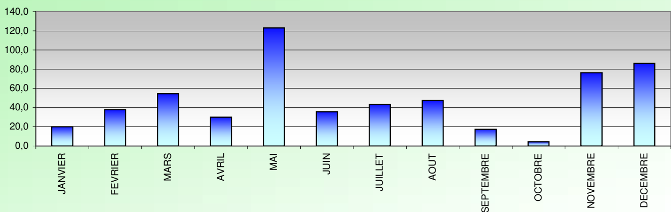
PRECIPITATIONS (mm) 2017
