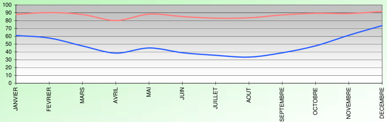
HUMIDITE RELATIVE (%) 2017
