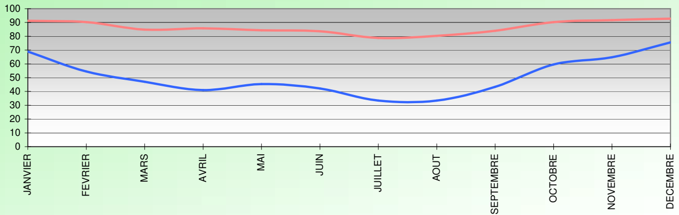
HUMIDITE RELATIVE (%) 2020
