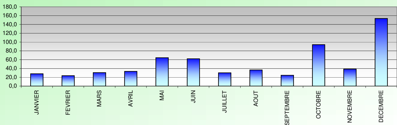
PRECIPITATIONS (mm) 2020
