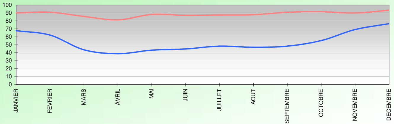
HUMIDITE RELATIVE (%) 2021
