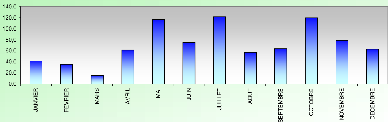
PRECIPITATIONS (mm) 2021
