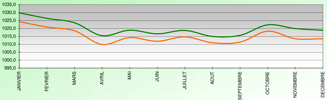
PRESSION RELATIVE (hPa) 2022
